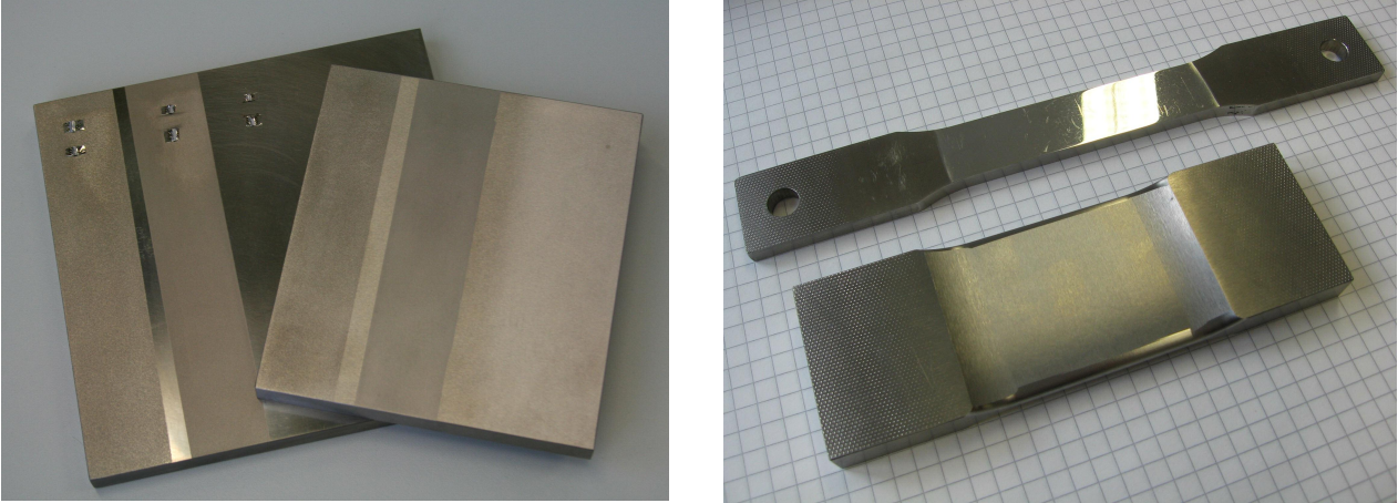
FIGURE 3. left picture: shot peened specimens made of IN718 (upper) and Ti6Al4V (below); right picture: tensile test specimen for measuring SAW parallel and perpendicular to stress direction
