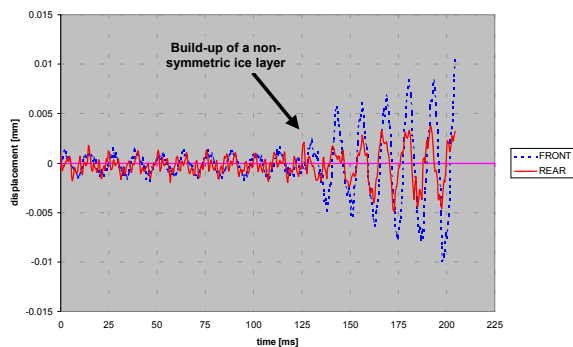
Figure 11 Icing test: Transient displacements at DOF corresponding to the sensors for a selected speed band
