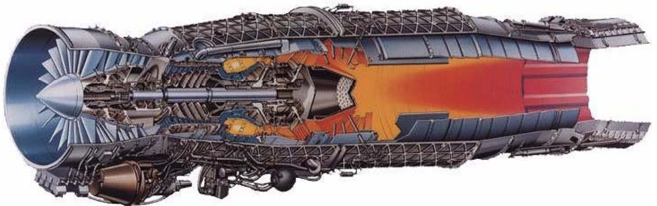
Figure 1 Engine EJ200
