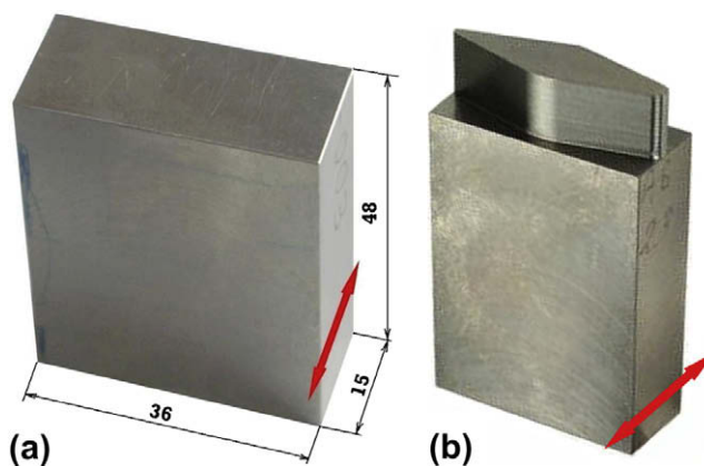
Fig. 1. Samples with prismatic (a) and blade like (b) geometry. The arrows indicate the direction of friction motion.
