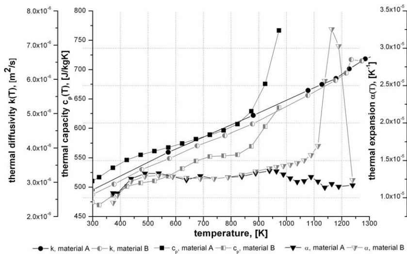
Fig. 6. Measured material's properties, thermal expansion was measured by dilatometry, heat capacity by differential scanning calorimetry and thermal diffusivity by laser flash method.
